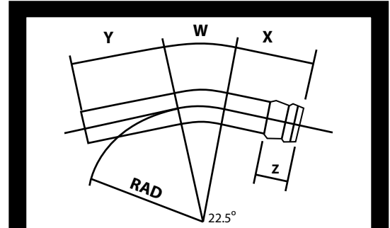
22.50 DEGREE BENDS
