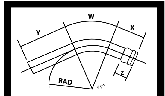
45 DEGREE BENDS
