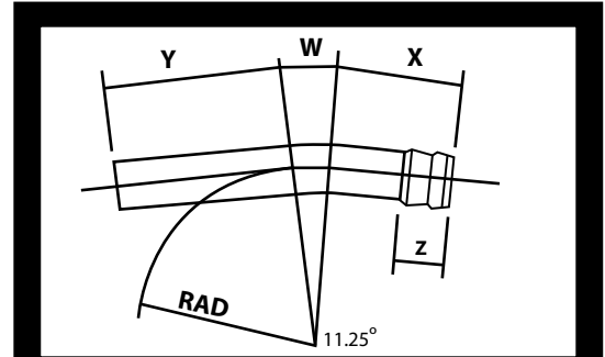
11.25 DEGREE BENDS
