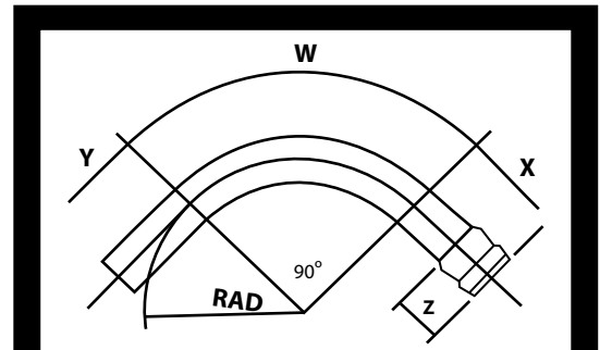
90 DEGREE BENDS
